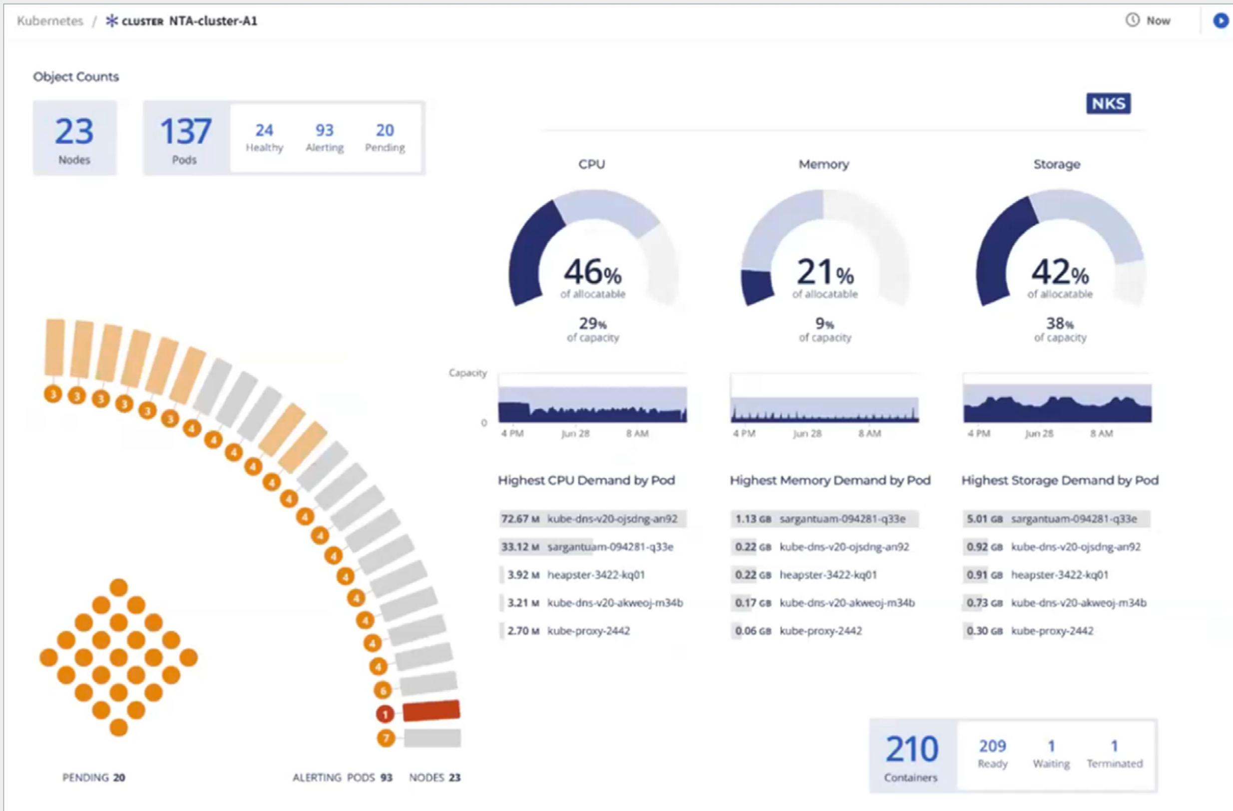
Figure 3) Exploded view of Kubernetes cluster information.
