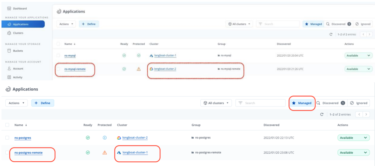
Figure 13) MySQL migrated to the destination cluster.
